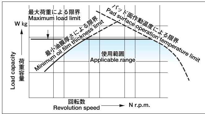
図7-回転数と荷重容量線図 Fig. 7-Reference chart of revolution speed and load capacity
